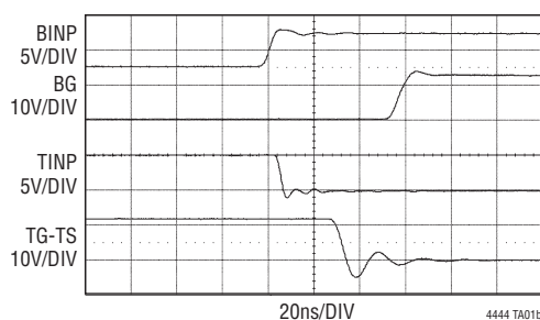
LTC4444 Driving a 1000pF Capacitive Load
