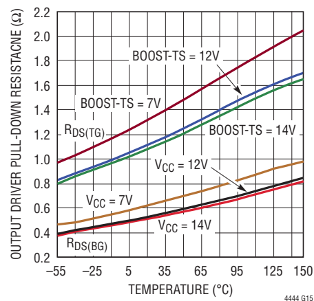
Output Driver Pull-Down Resistance vs Temperature
