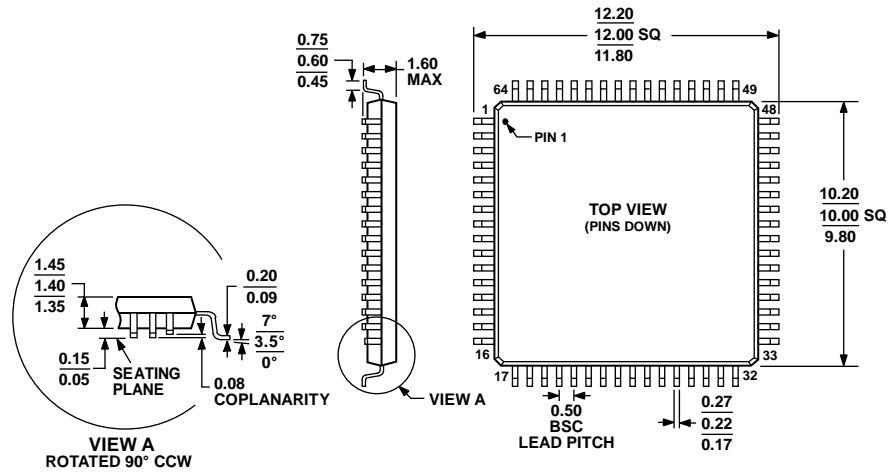
Figure 32. 64-Lead Low Profile Quad Flat Package [LQFP] (ST-64-2) Dimensions shown in millimeters
