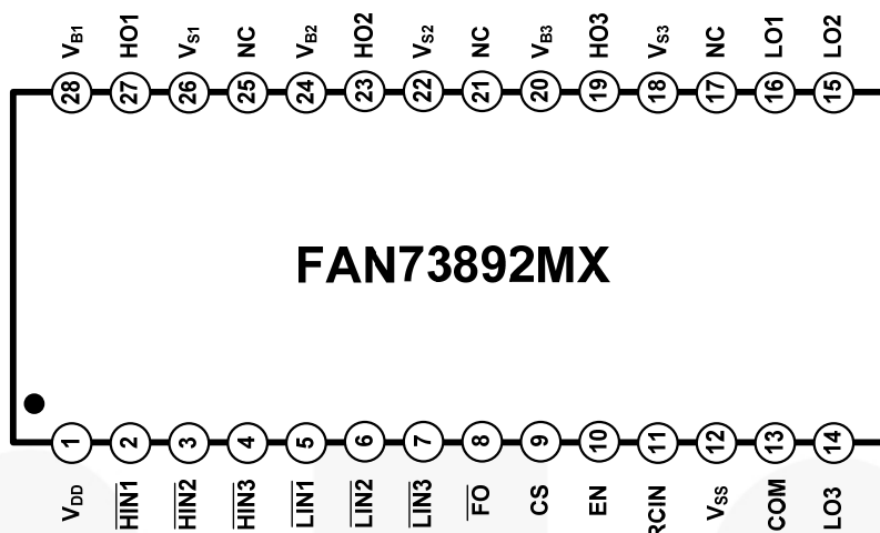
Figure 3. Pin Assignments
