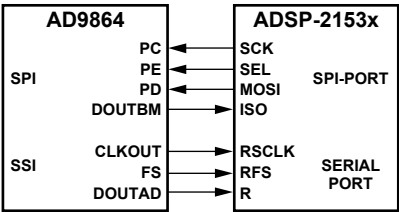
Figure 37. Example of AD9864 and ADSP-2153x Interface
