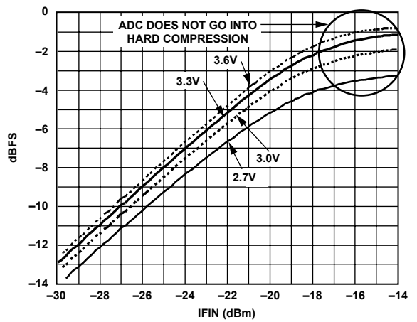
Figure 10. Gain Compression vs. IFIN
