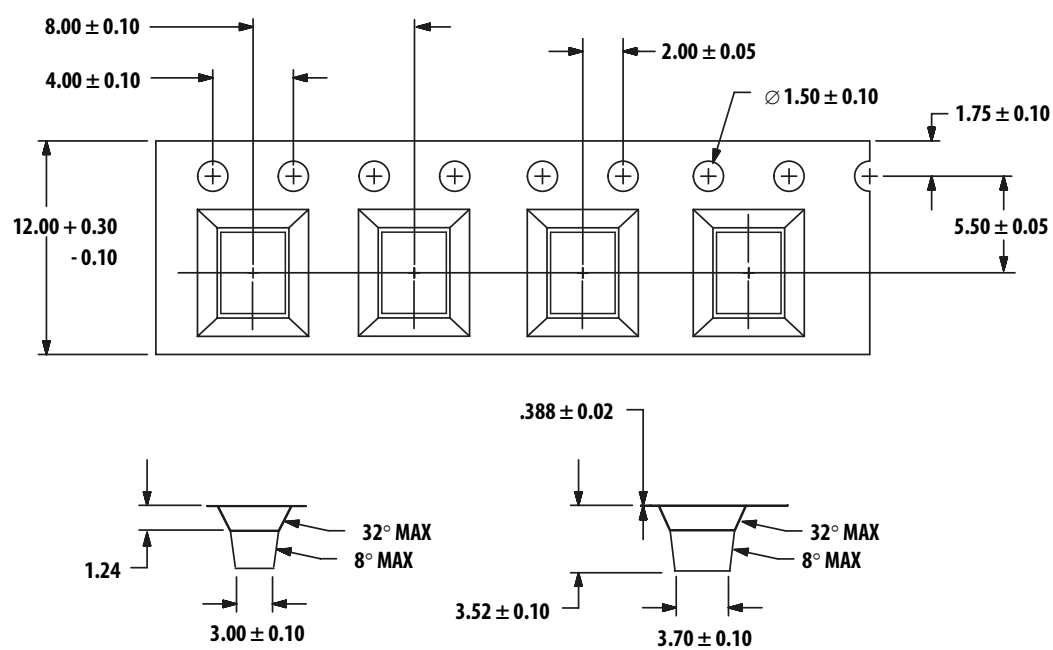
Figure 11. Tape Dimensions
