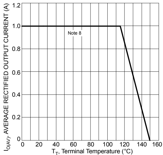
Fig. 4 Forward Current Derating (Note 4)
