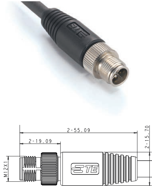
M12 Pin Connector Cable Assembly
