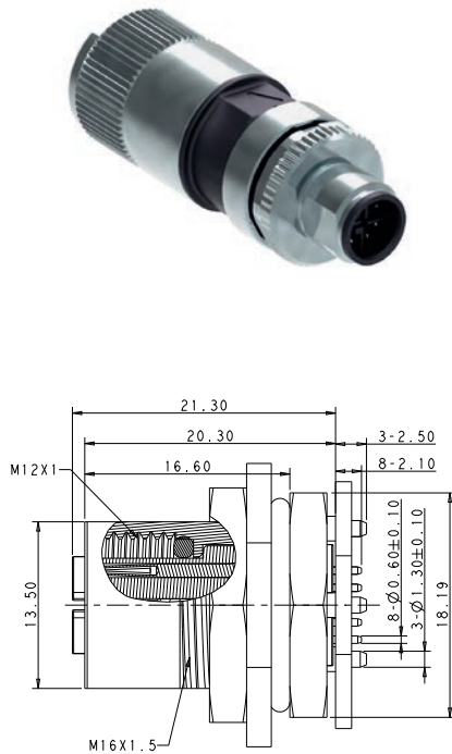
M12 X-Coded PCB Connector
