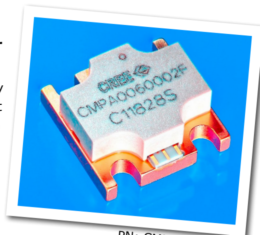
PN: CPMA0060002F Package Type: 780019
