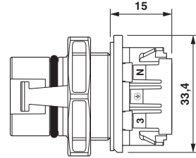
Dimensional drawing
