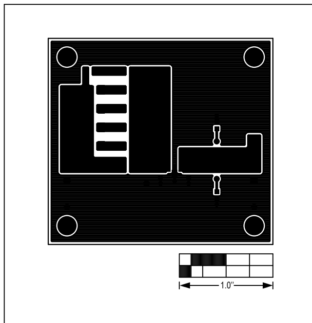
Figure 3. MAX14626 EV Kit PCB Layout—Component Side
