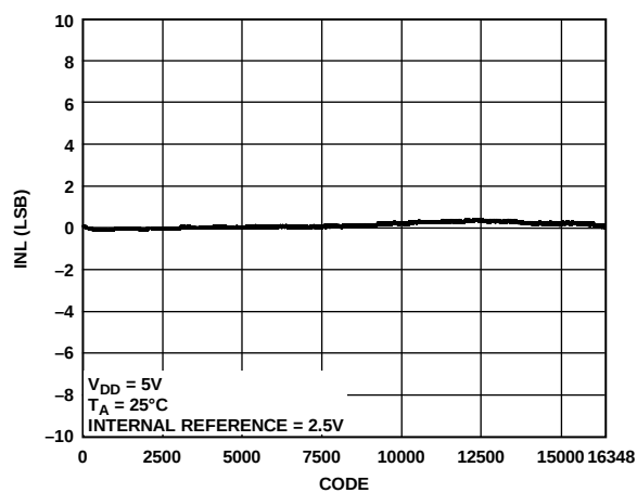
Figure 16. AD5685R INL
