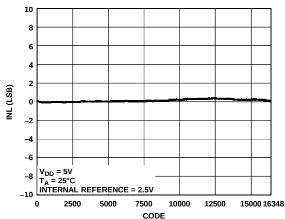
Figure 16. AD5685R INL
