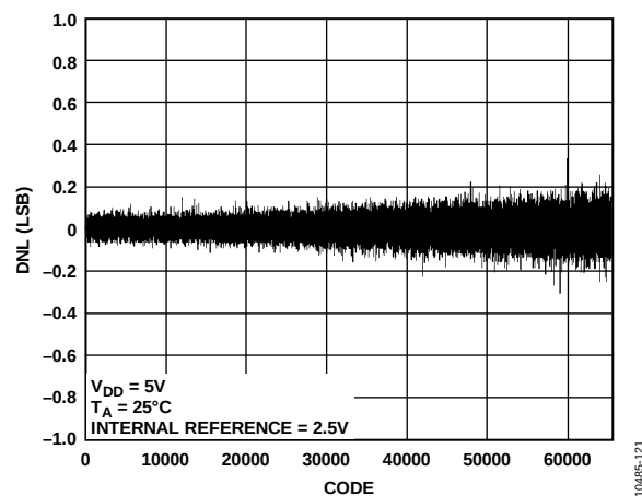
Figure 18. AD5686R DNL
