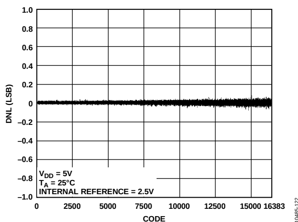
Figure 19. AD5685R DNL
