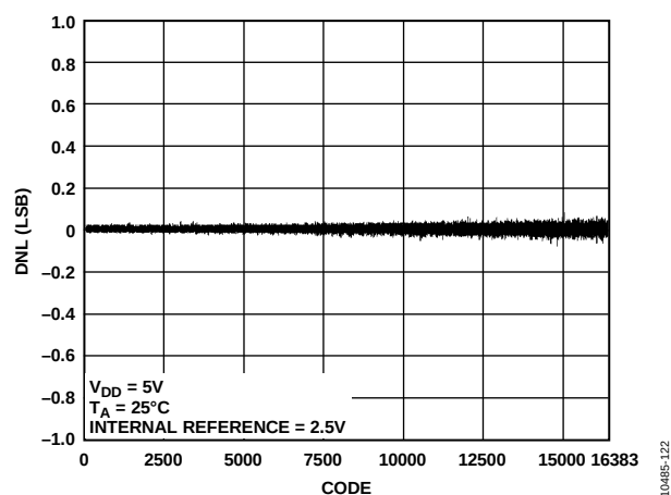
Figure 19. AD5685R DNL
