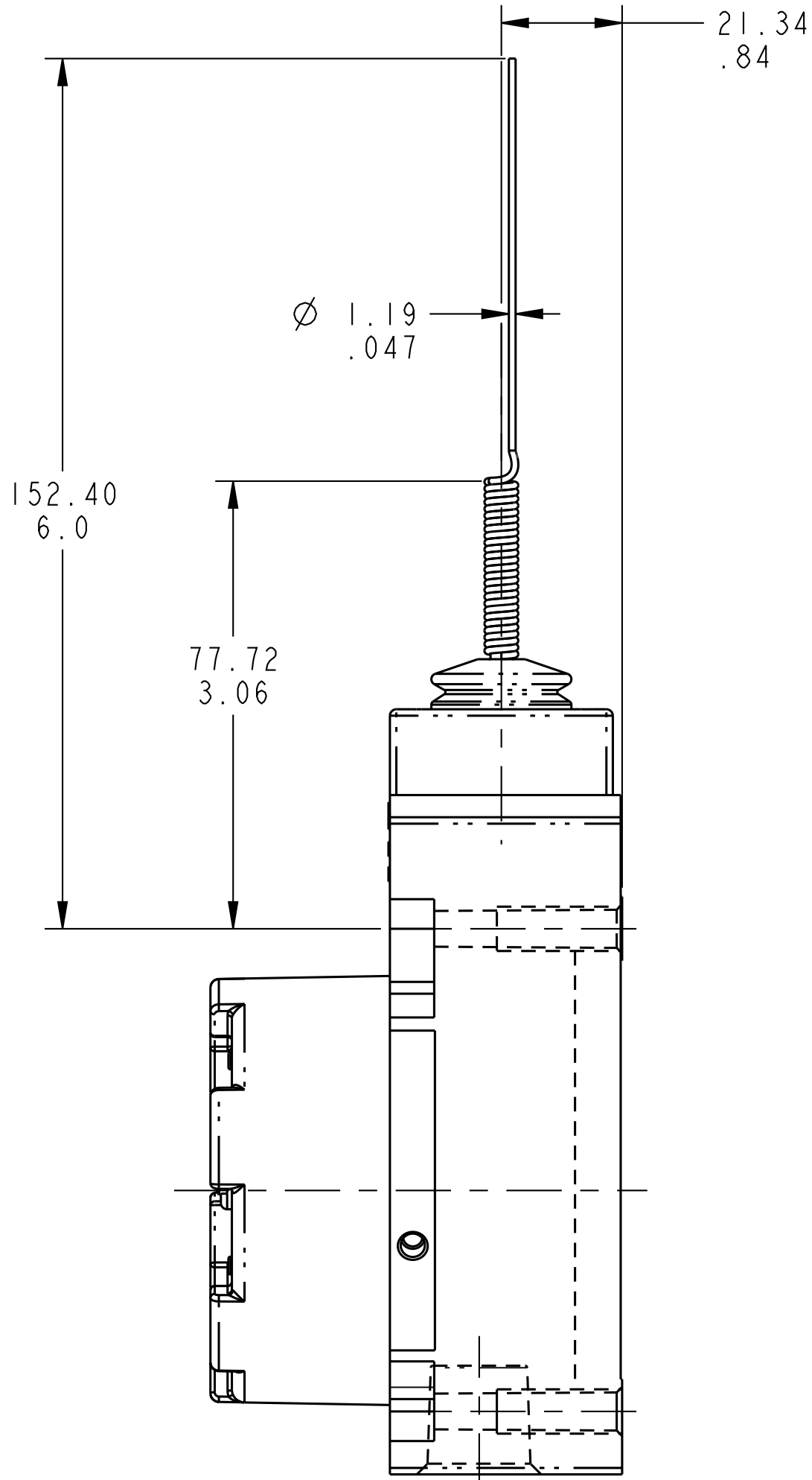
WIRE EXTENSION TYPE 8A ACTUATOR
