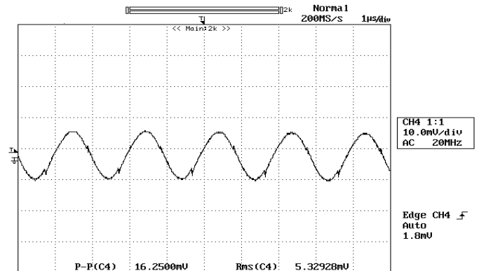
Figure 12: Output ripple & noise at 12Vin, 5.0V/20A out
