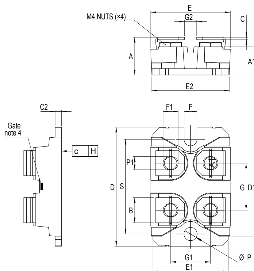
Figure 8. ISOTOP™ package outline
