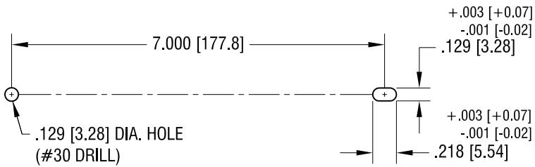
SUGGESTED MOUNTING DETAIL
