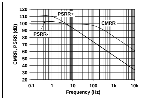
FIGURE 2-28: CMRR, PSRR vs. Frequency.
