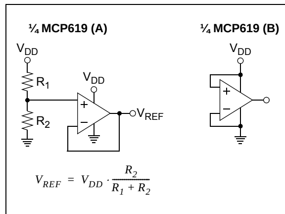
FIGURE 4-7: Unused Op Amps.
