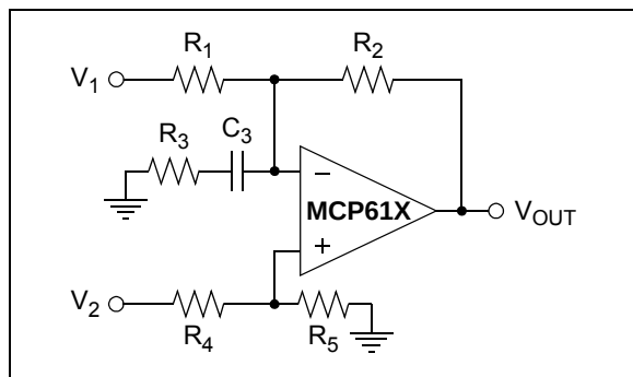
FIGURE 4-3: Example Circuit for Calculating DC Offset.
