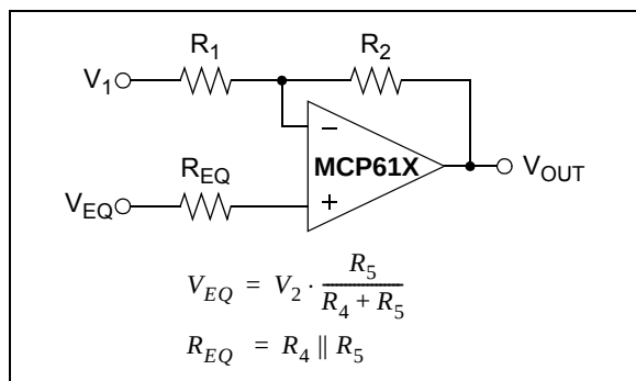
FIGURE 4-4: Equivalent DC Circuit.
