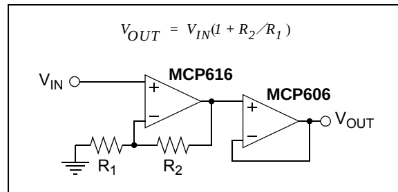
FIGURE 4-12: Precision Gain with Good Load Isolation.
