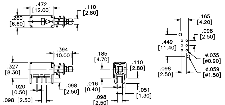
MECHANICAL OUTLINE
