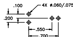
P.C. BOARD LAYOUT
