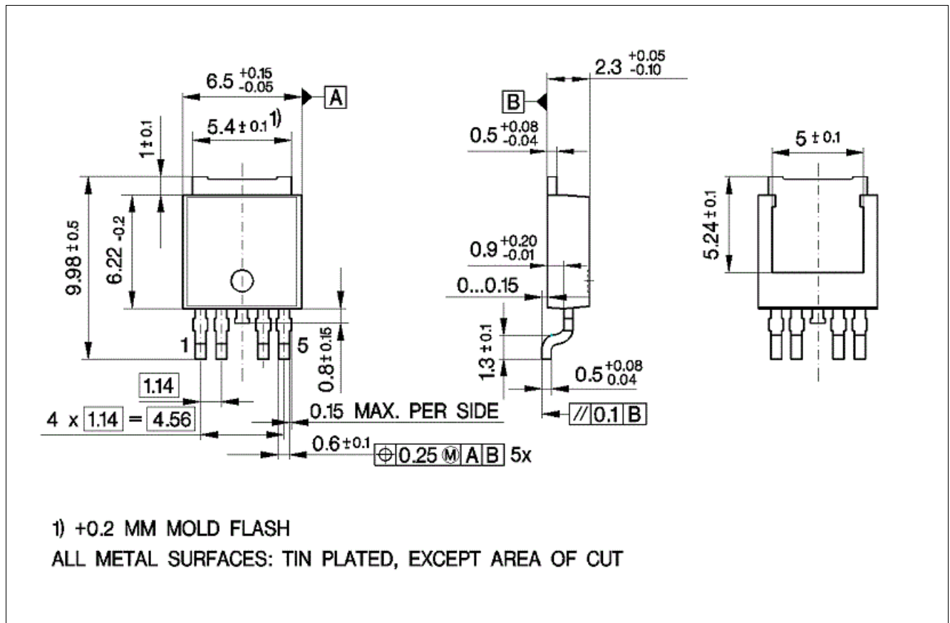
PG-T0252-5 (Transistor Outline Package)
