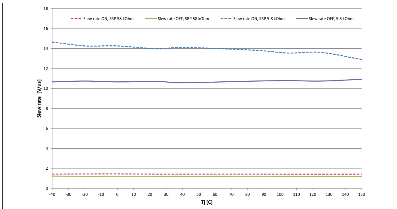
Figure 28 Typical slew rate vs. T_j (-40..150°C) @ R_{SRP}=5.8\text{k}\Omega and 58kΩ
