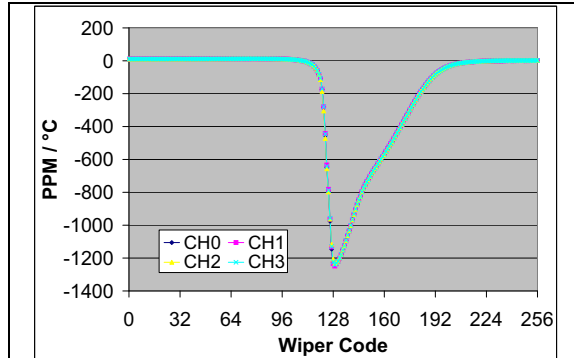
FIGURE 2-60: 50 kΩ – R_{WB} PPM/ ^\circ\text{C} vs. Wiper Setting. ( R_{BW(\text{code}=n, 125^\circ\text{C})} - R_{BW(\text{code}=n, -40^\circ\text{C})} / R_{BW(\text{code}=256, 25^\circ\text{C}) / 165^\circ\text{C}} * 1,000,000 ) ( V_{DD} = 3.0\text{V} , I_W = 48\text{ }\mu\text{A} ).
