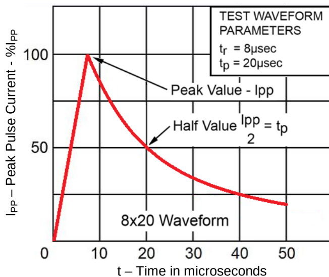
FIGURE 2 Pulse Waveform
