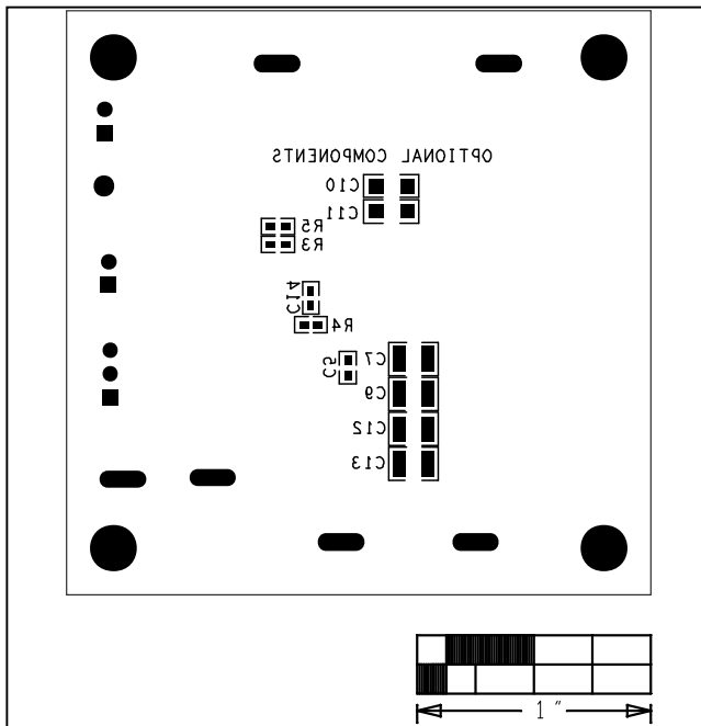
Figure 2. MAXM17504 EV Kit Component Placement Guide—Solder Side
