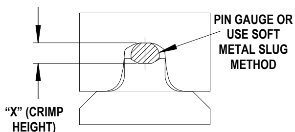
CRIMP PROFILE
