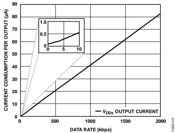
Figure 14. Current Consumption per Output vs. Data Rate for 2.5 V, EN_x = \text{High Operation}
