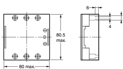
With Terminal Cover
