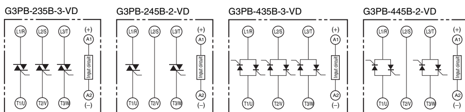
Terminal Arrangement/Internal Circuit Diagram
