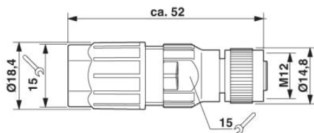
Dimensioned drawing
