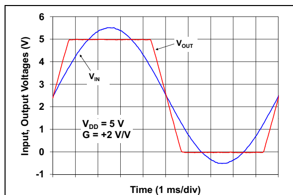
FIGURE 2-32: The MCP6491/2/4 Shows No Phase Reversal.
