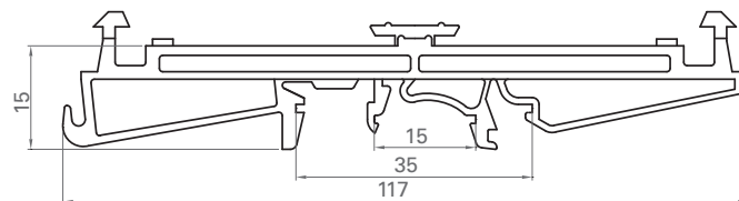
DIN RAIL MOUNTING FOOT (110mm)
