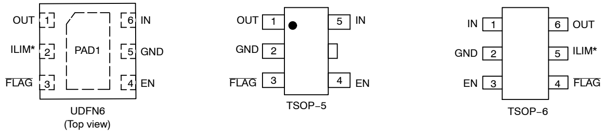
Figure 2. Pin Connections
