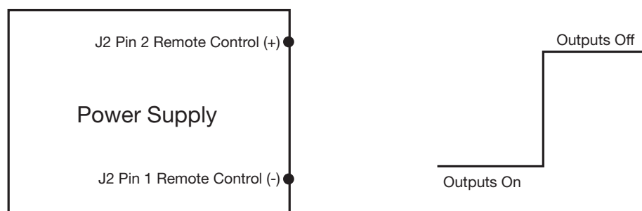
Figure 9 - Remote On/Off
