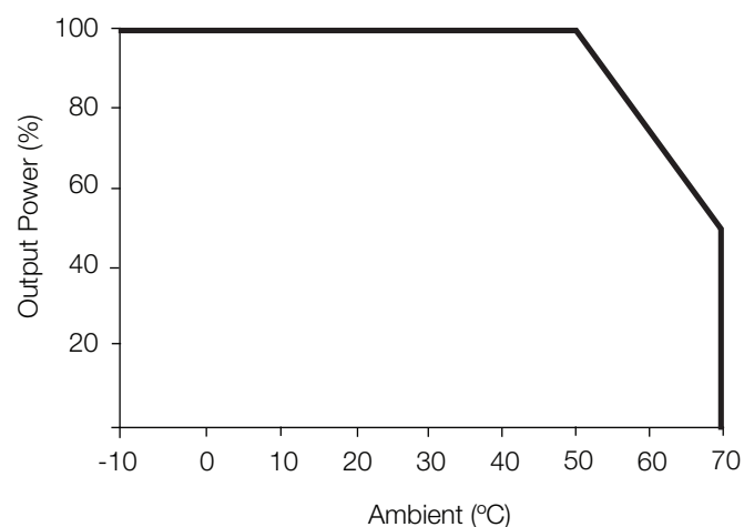
Figure 10 - LCL150 & LCL300
