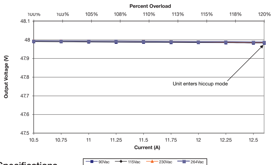
Figure 4 - LCL500PS48
