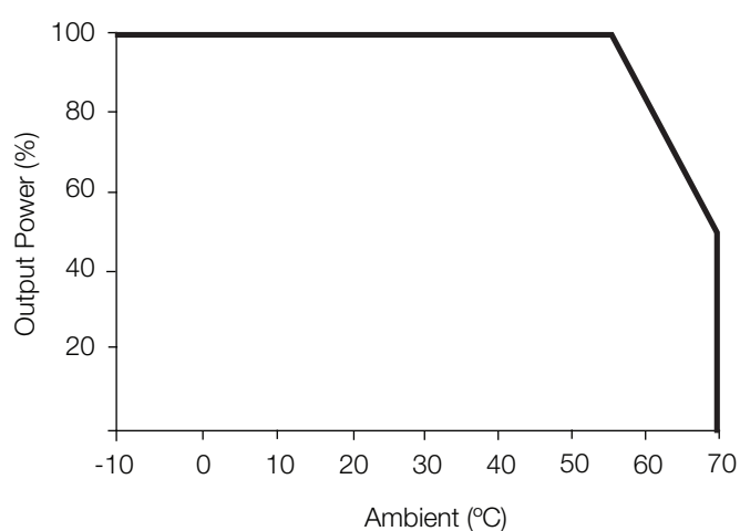
Figure 11 - LCL500
