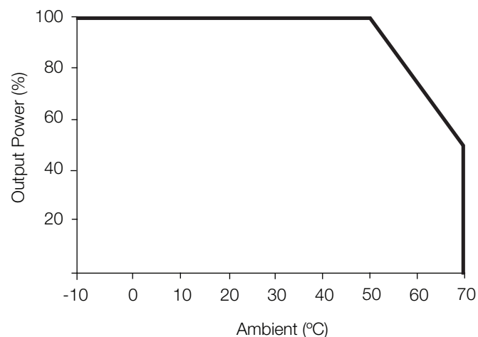
Figure 10 - LCL150 & LCL300
