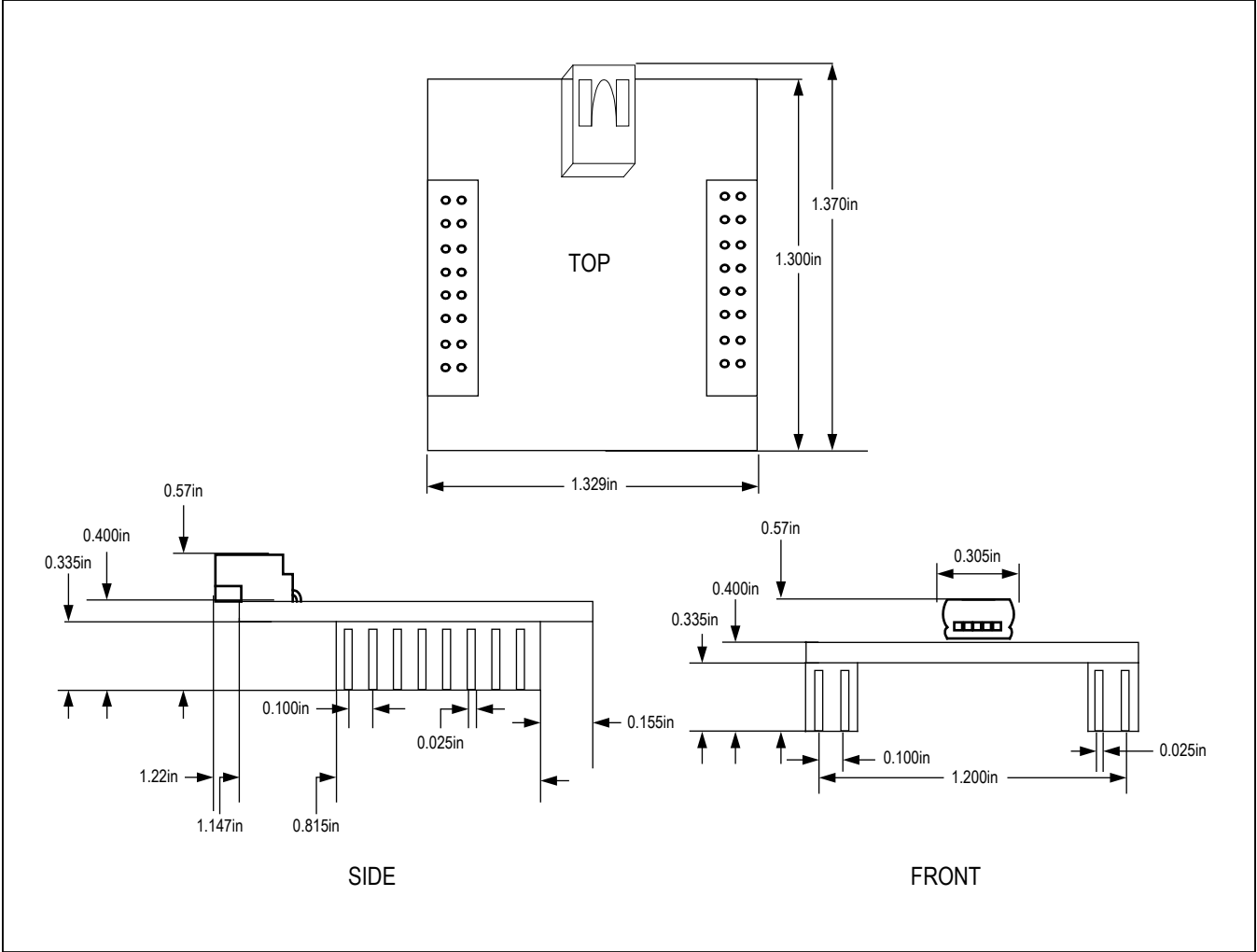
Figure 6. DS3900H2 Dimensions
