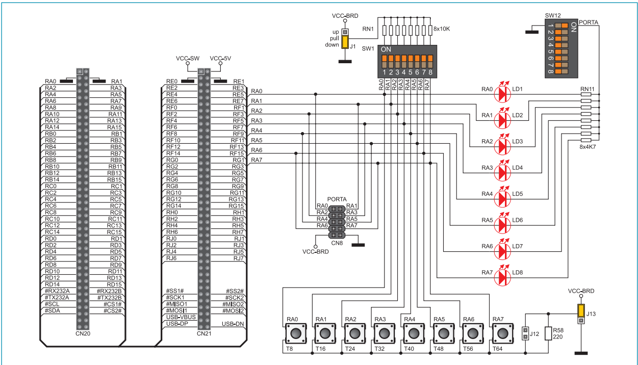
Figure 17-1: I/O ports
