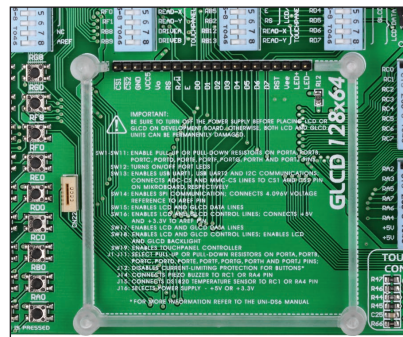
Figure 15-2: GLCD connector
