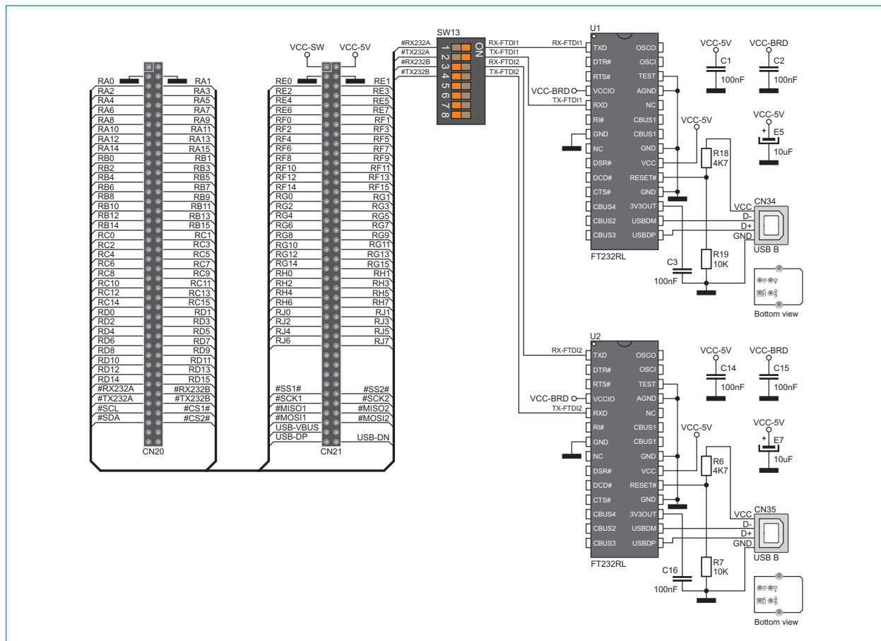
Figure 5-1: USB UART modules
