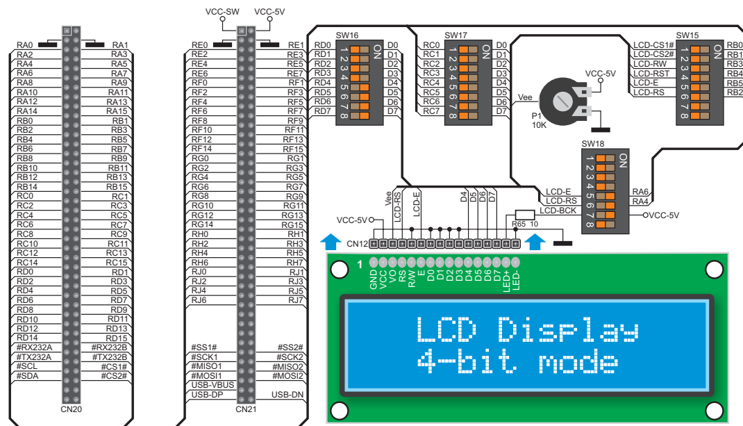
Figure 14-2: Alphanumeric 2x16 LCD display
