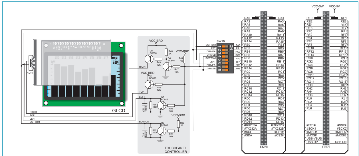
Figure 16-1 shows how to place a touch panel over a GLCD display. Make sure that the flat cable is to the left of the GLCD, as shown in Figure 1D.
