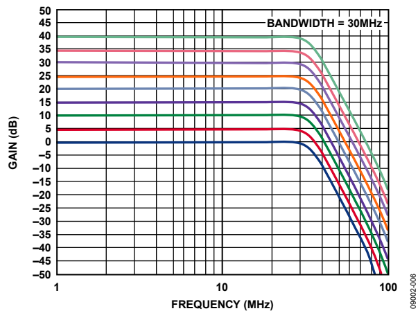
Figure 6. Gain vs. Frequency by V_{\text{GAIN}} (Bandwidth Setting = 30 MHz)
