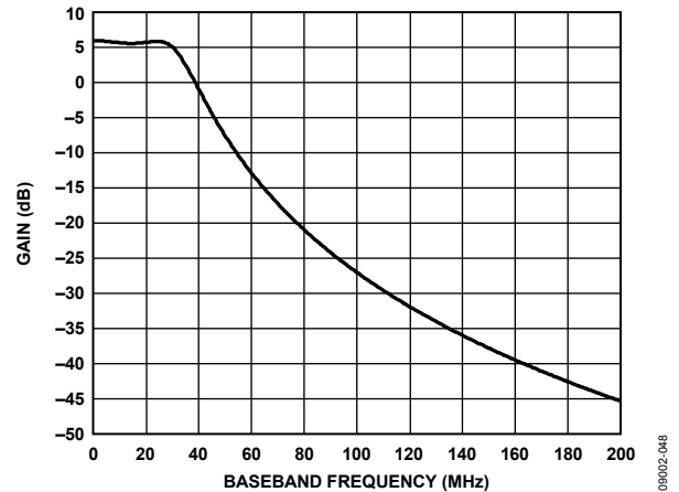
Figure 57. Third-Order Baseband Filter Response
