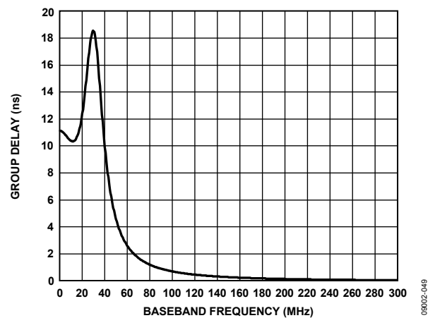
Figure 58. Third-Order Baseband Filter Group Delay Response
