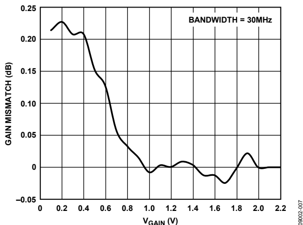
Figure 7. Gain Matching vs. V_{\text{GAIN}} (Bandwidth Setting = 30 MHz)
