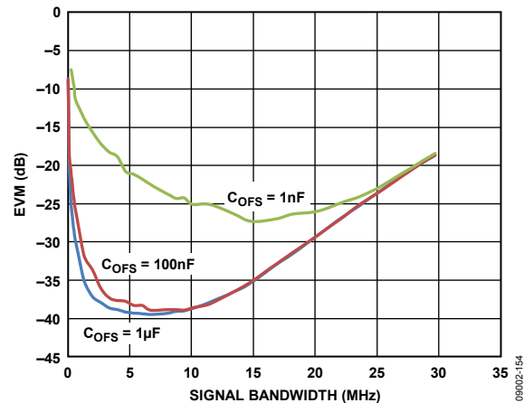
Figure 54. EVM vs. Signal BW over C_{OFS} Values
