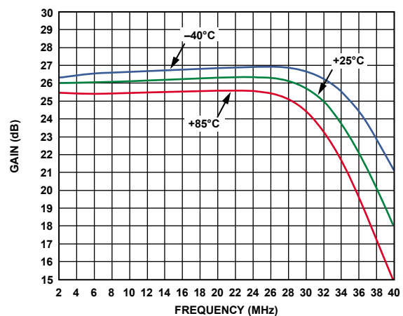
Figure 13. Frequency Response over Temperature (Gain = 26 dB, Bandwidth Setting = 30 MHz)
