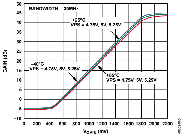
Figure 5. In-Band Gain vs. V_{\text{GAIN}} over Supply and Temperature (Bandwidth Setting = 30 MHz)
