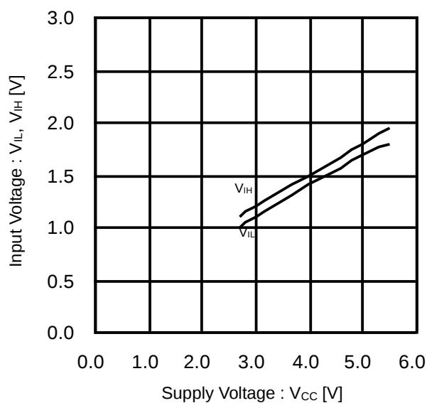
Figure 15. Input Voltage vs Supply Voltage
