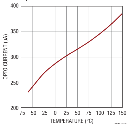
Opto-Driver Sink Current
