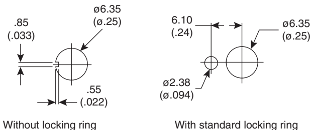
PANEL MOUNTING
