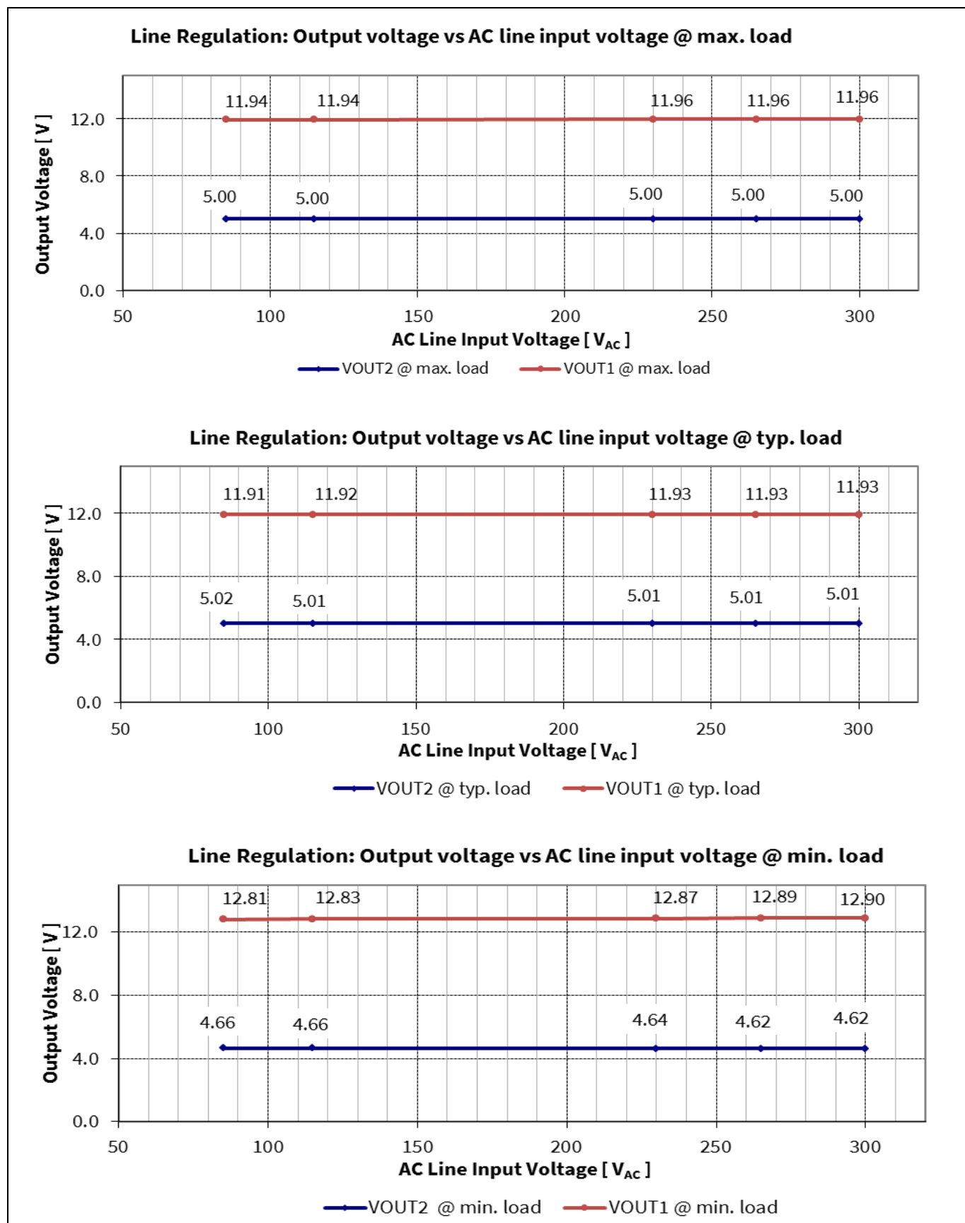
Figure 10 Line regulation: V_{OUT} vs AC-line input voltage
