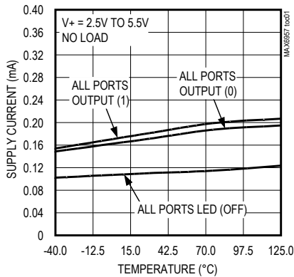
OPERATING SUPPLY CURRENT vs. TEMPERATURE
