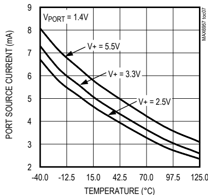
GPO SOURCE CURRENT vs. TEMPERATURE (OUTPUT = 1)
