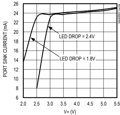
LED DRIVER SINK CURRENT vs. V+
