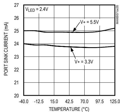
LED DRIVER SINK CURRENT vs. TEMPERATURE
