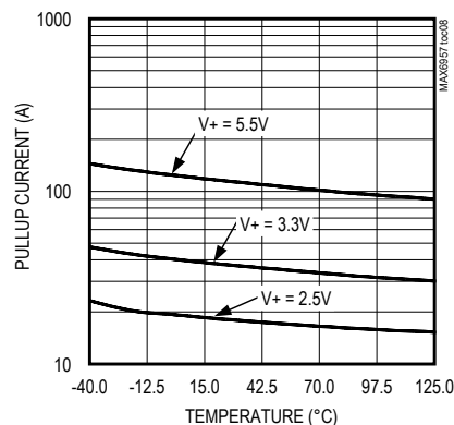
GPI PULLUP CURRENT vs. TEMPERATURE
