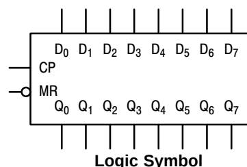
Logic Symbol
