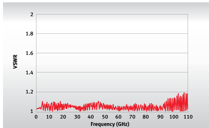
FIGURE 3: TYPICAL VSWR 1
