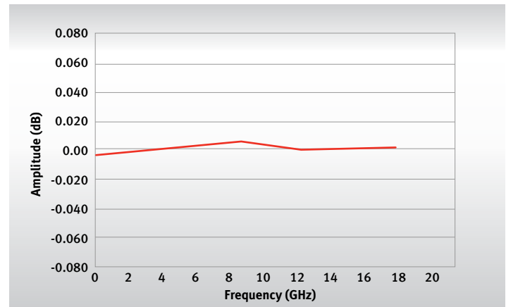
FIGURE 2: TYPICAL AMPLITUDE STABILITY WITH FLEXURE AND SHAKE 1
