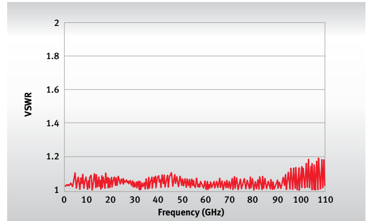
FIGURE 3: TYPICAL VSWR 1
