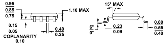
Figure 42. 8-Lead Mini Small Outline Package [MSOP] (RM-8)
