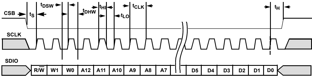
FIGURE 44. SPI WRITE
