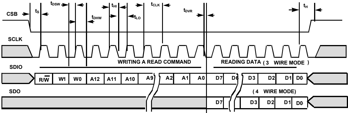
FIGURE 45. SPI READ
